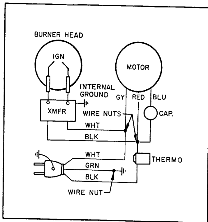
Figure 2. Wiring Diagram
