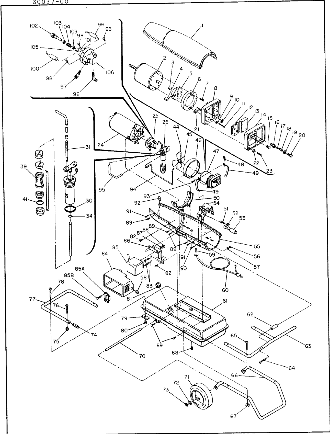
Figure 4. Heater, Exploded View
