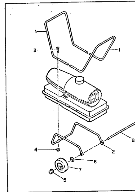
Figure 16. Handles and Wheels
