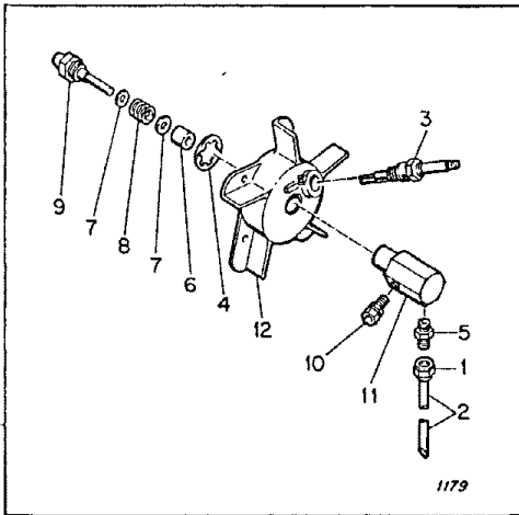
Figure 15. Burner Head Assembly
