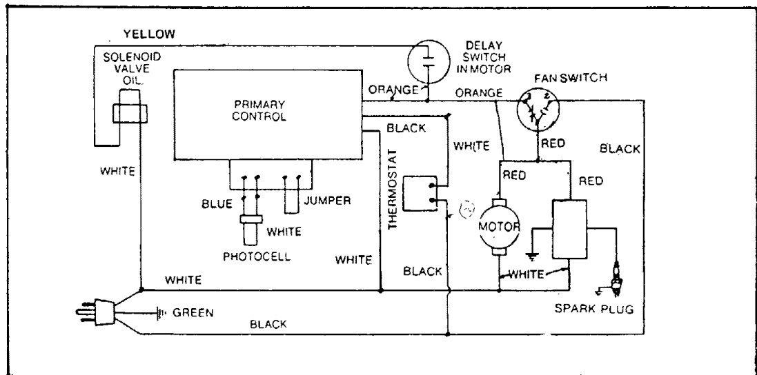
Figure 1. Wiring Diagram
