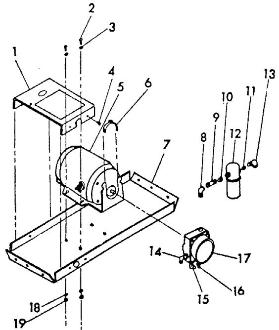
Figure 6. Motor and Pump Assembly
