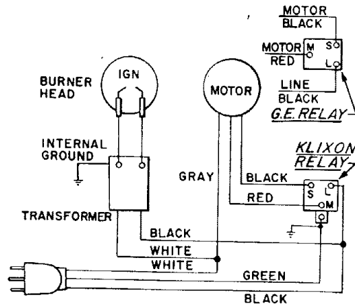
Wiring Diagram for 75,000 BTU Heater
