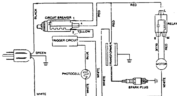
Wiring Diagram
