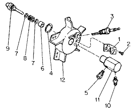
Figure 14. Burner Head Assembly
