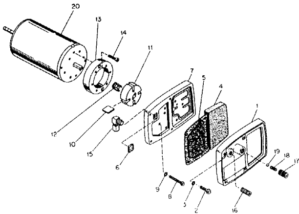
Figure 15. Motor Package Assembly
