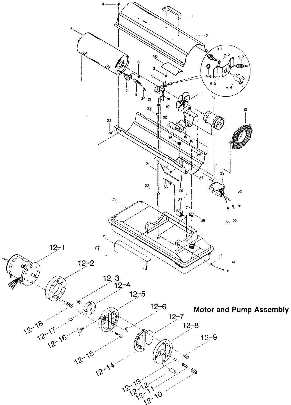
Figure 1 - Replacement Parts Illustration for Heater Model F50E
