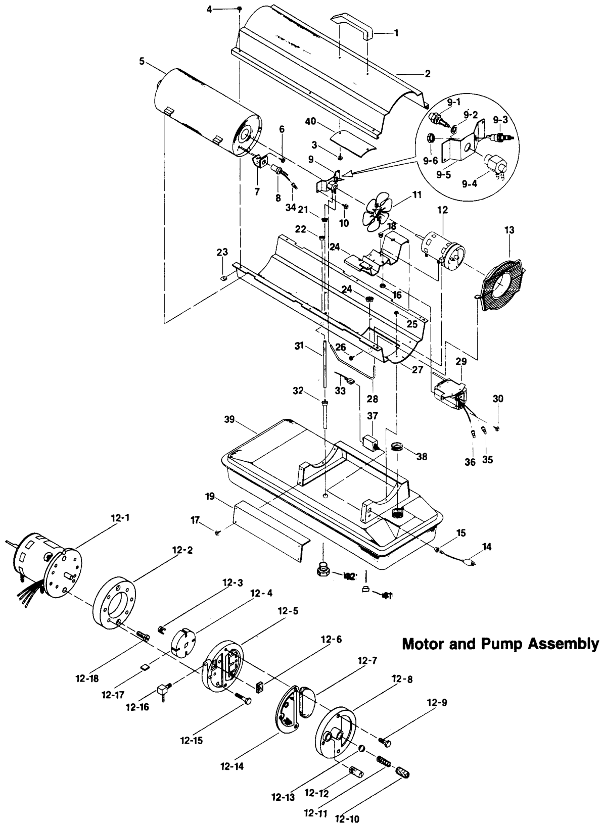
Figure 1 - Replacement Parts Illustration for Heater Model B50D
